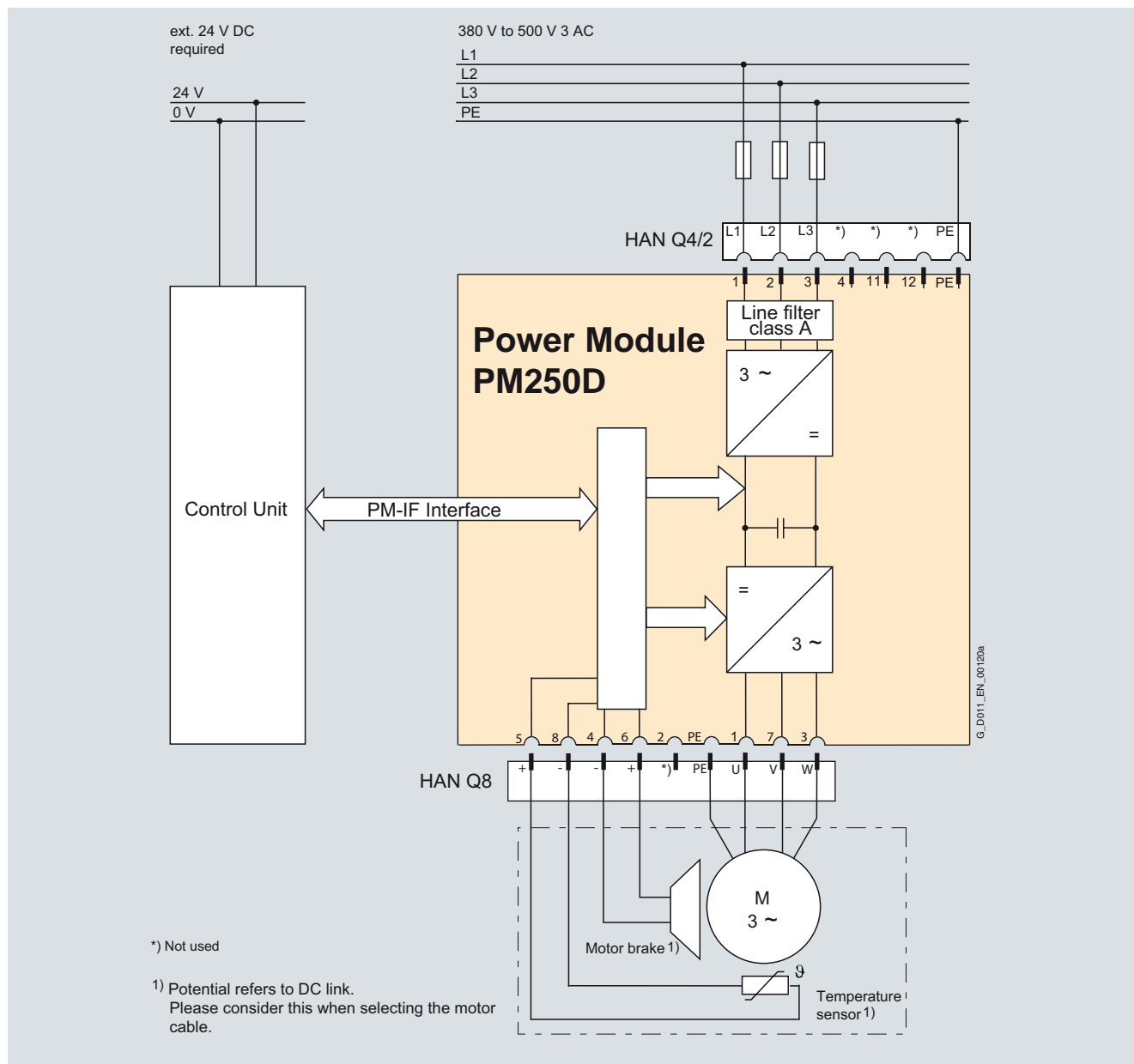
Connection diagram for PM250D Power Module with integrated class A line filter
