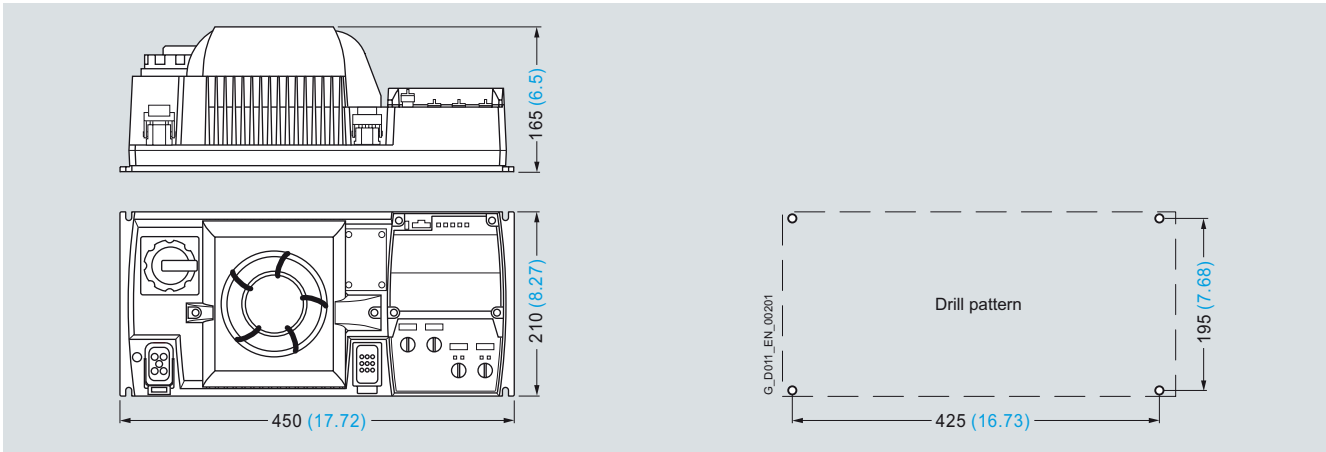
SINAMICS G110D, frame size FSB with integrated class A line filter and maintenance switch
